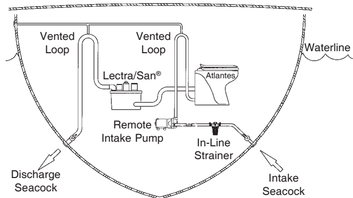
Atlantes with Remote Intake Pump installed below waterline.
