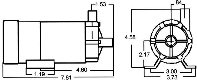
SERIES X30 (hose)
