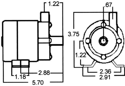
SERIES X5, X10 (hose)
