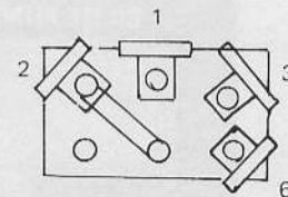
BILGE PUMP LIGHTED SWITCH 44960-0000
