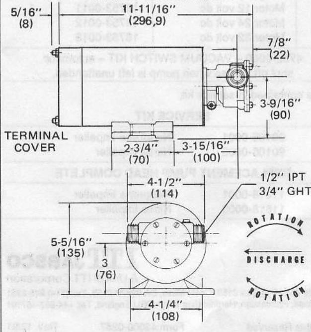
DIMENSIONAL DRAWING INCHES (MILLIMETRES)
