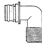
50645-1000 (1 PAIR) SNAP-IN PORT X 1/2" - 14 MALE PIPE 90° ELBOW
