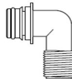
30655-1000 SNAP-IN PORT x 1/2" MALE QEST. 90° ELBOW
