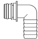
30642-1000 SNAP-IN PORT x 3/4" HOSE BARB 90° ELBOW
