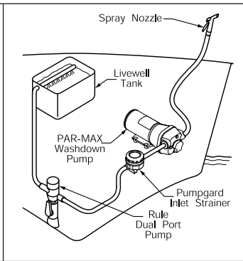
Fig. 2 31605-Series w/Rule® Dual Port
