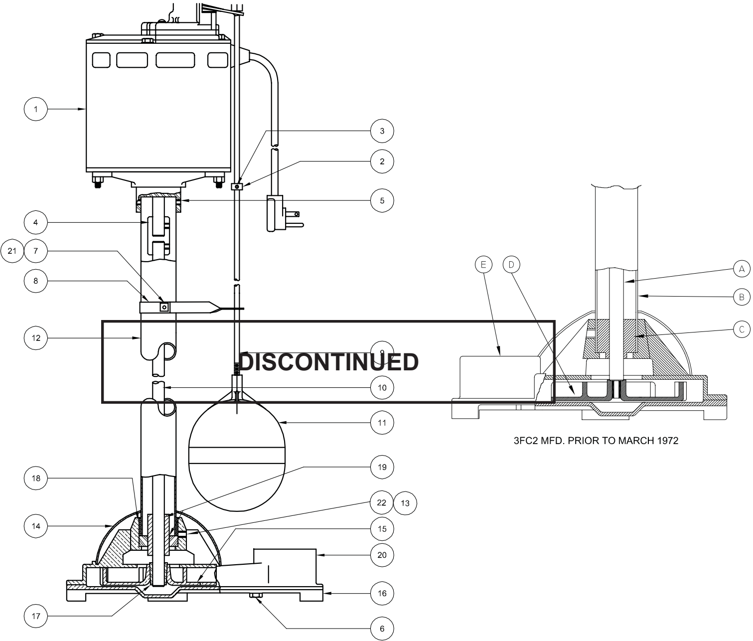
PUMP CAT. No. 3FC2
